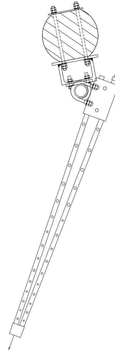
PROPOSED LOG PERIODIC Tx ANTENNA @ 13.5m MEAN 200°
