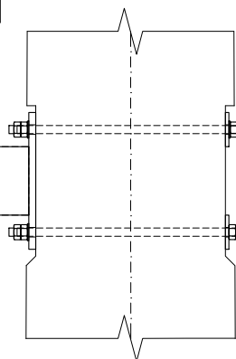
DETAIL H - Rx ANTENNA MOUNT Scale 1:10
